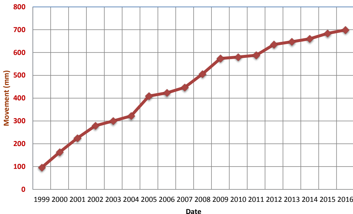
Figure A1: HUB 98-17 Total Horizontal Ground Movement
