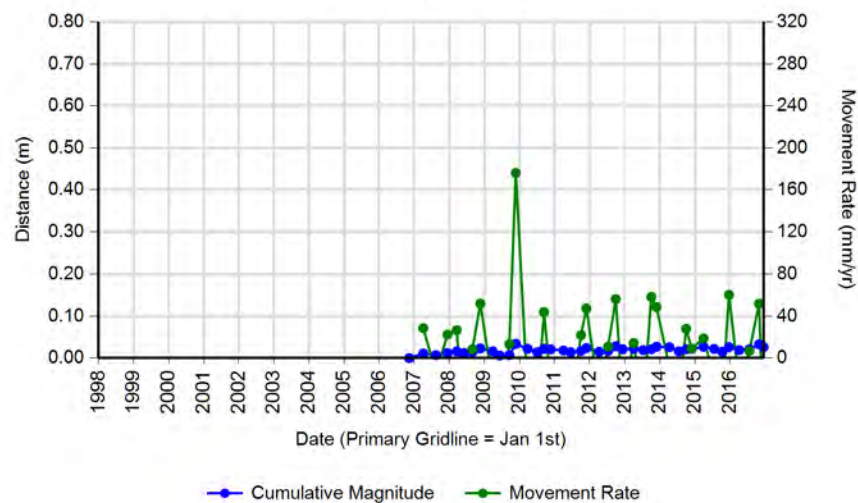
Horizontal Displacement
