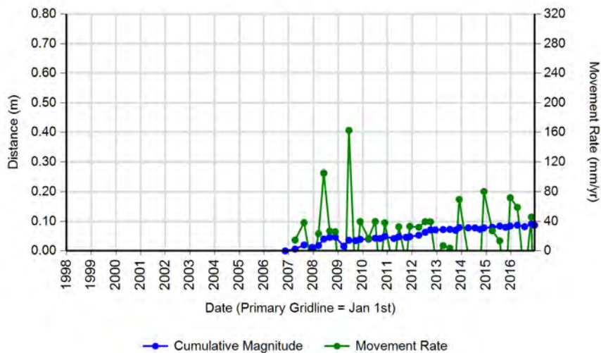
Horizontal Displacement
