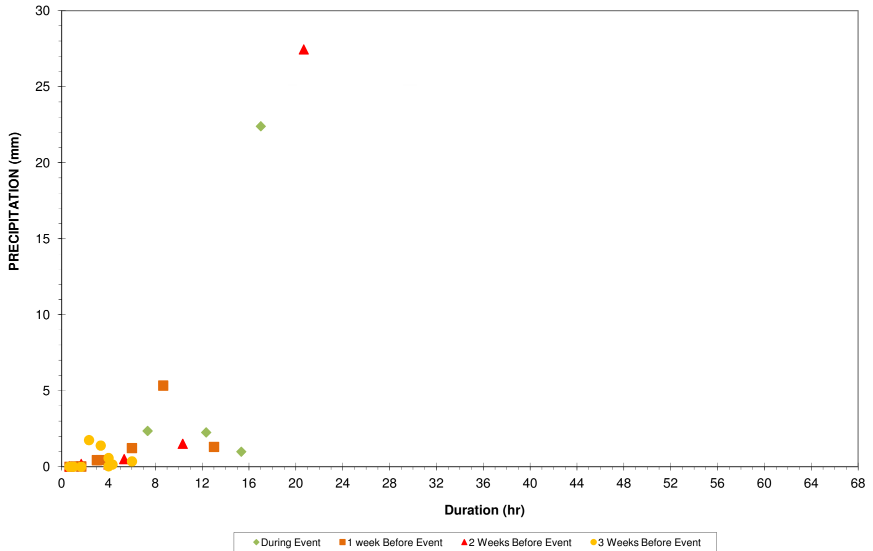
Figure F10 - Precipitation Events Around Ground Movement Event November 27 to 30 (WS1)
