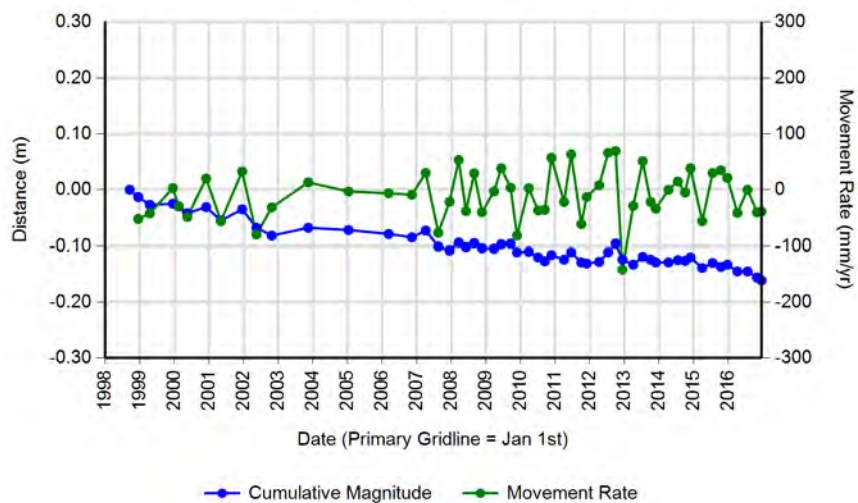
Vertical Displacement
