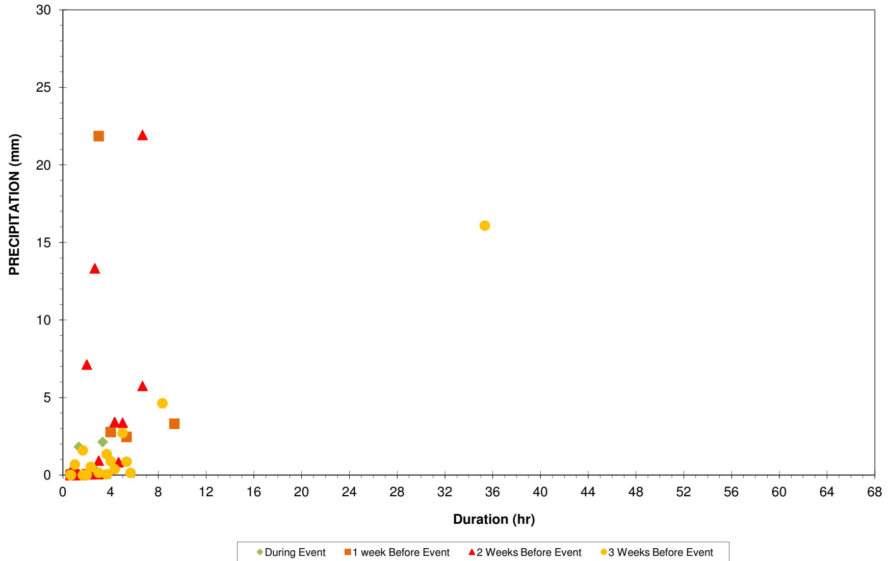
Figure F9 - Precipitation Events Around Ground Movement Event July 22 to 28 (WS1)
