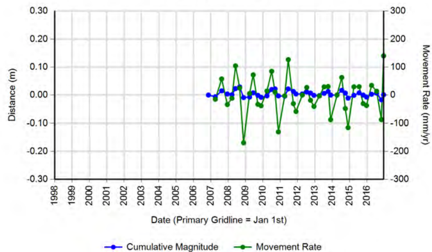
Vertical Displacement
