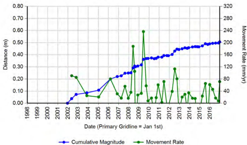
Horizontal Displacement
