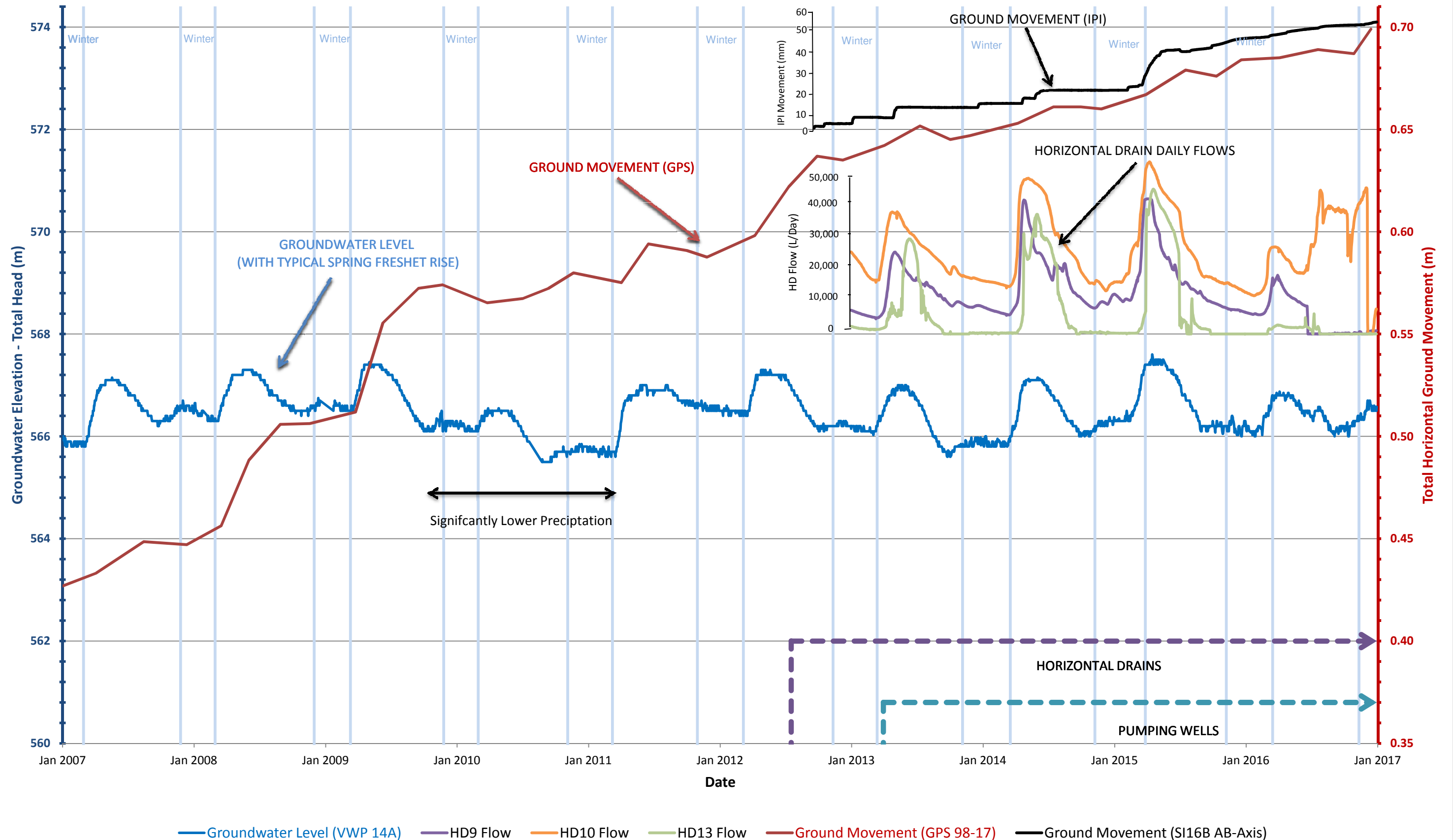
Figure G5 - Cumulative Ground Movement & Typical Background Groundwater Elevation
