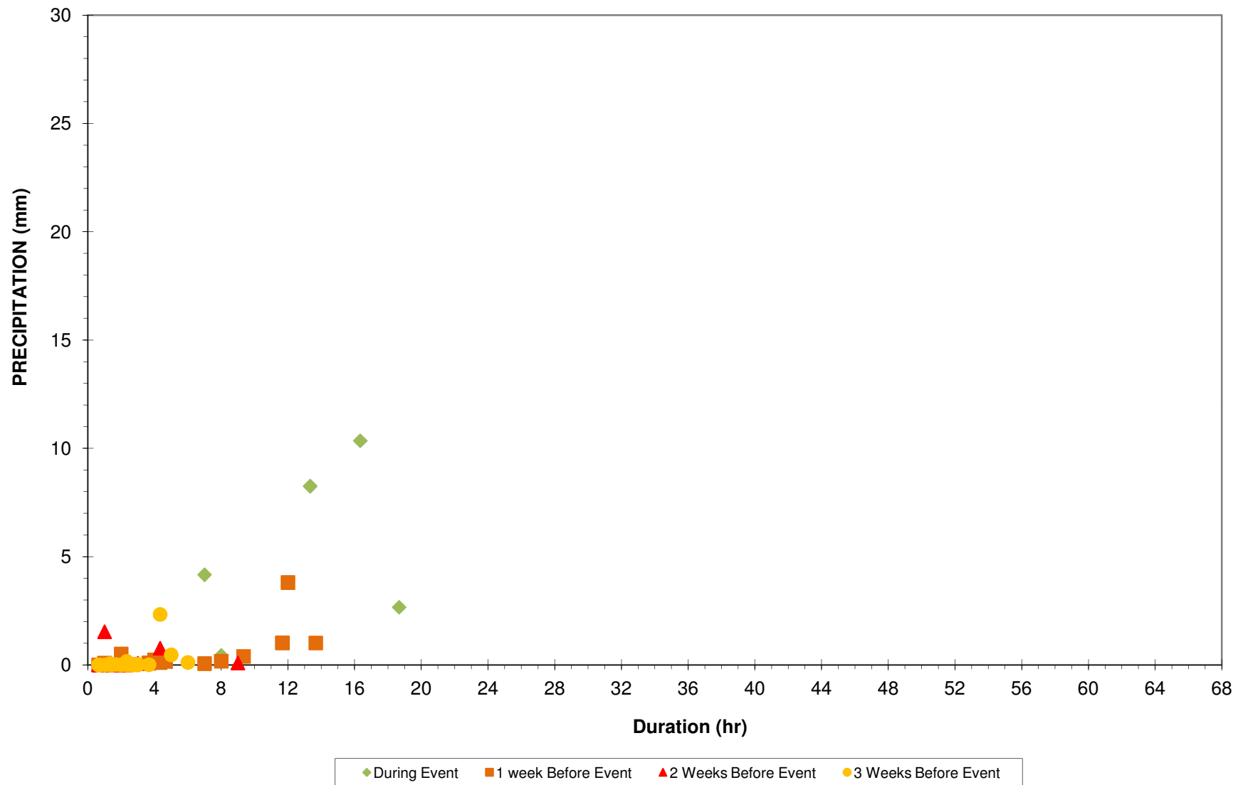
Figure F8 - Precipitation Events Around Ground Movement Event April 22 to 27 (WS1)
