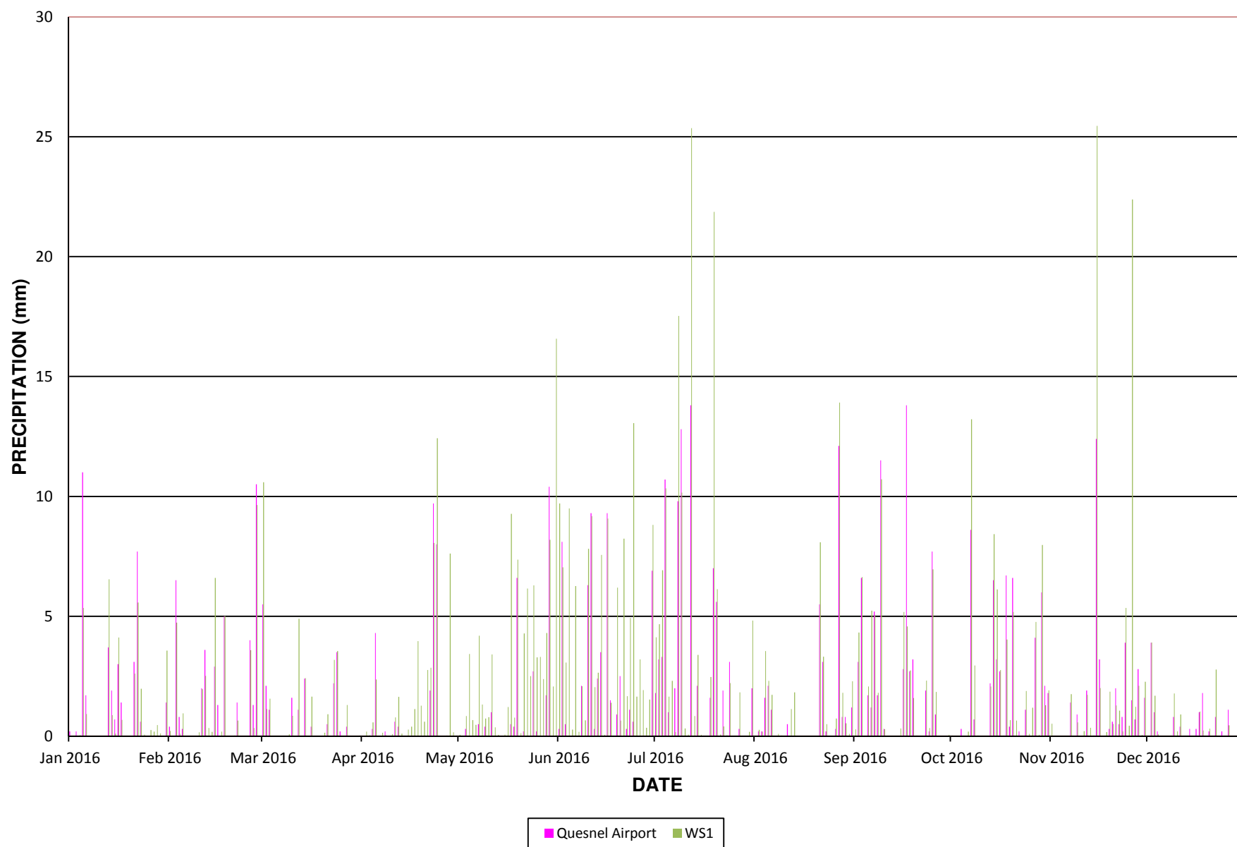
Figure F5 - Daily Precipitation 2016 (Environment Canada-Quesnel and WS1)
