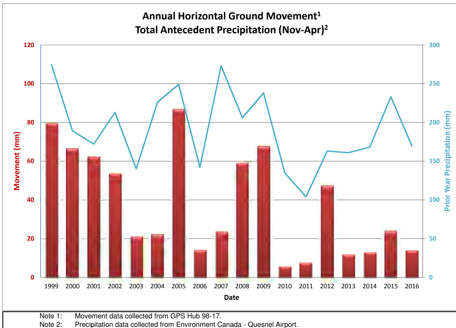
Figure G2 - Horizontal Movement Relative to Annual Precipitation
