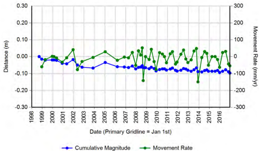
Vertical Displacement
