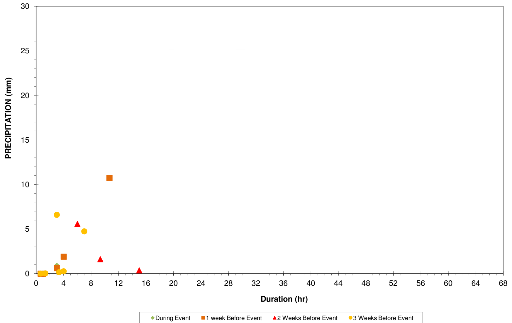
Figure F7 - Precipitation Events Around Ground Movement Event March 7 to 10 (WS1)
