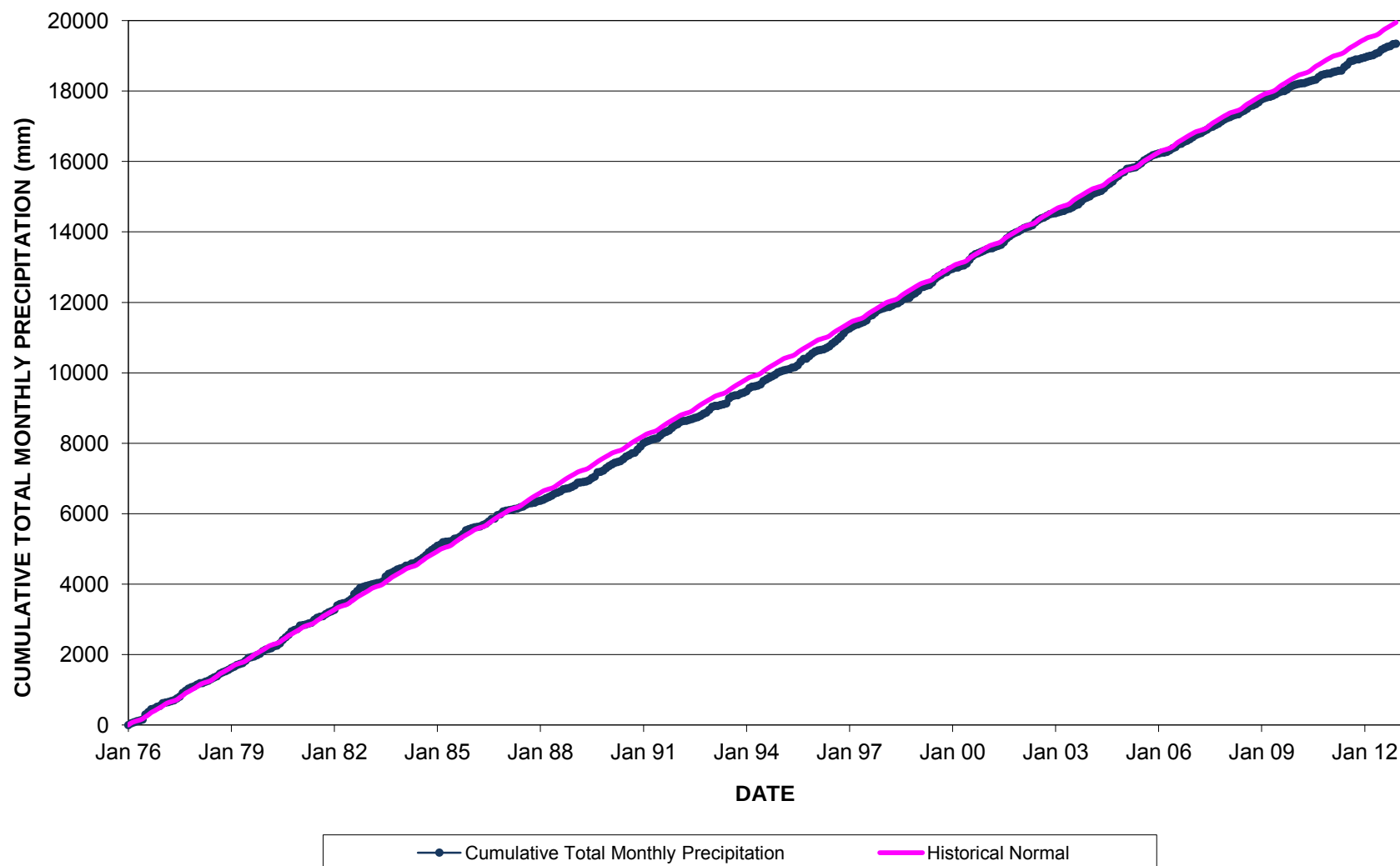
Figure F2 - Cumulative Total Monthly Precipitation (Environment Canada-Quesnel Station)
