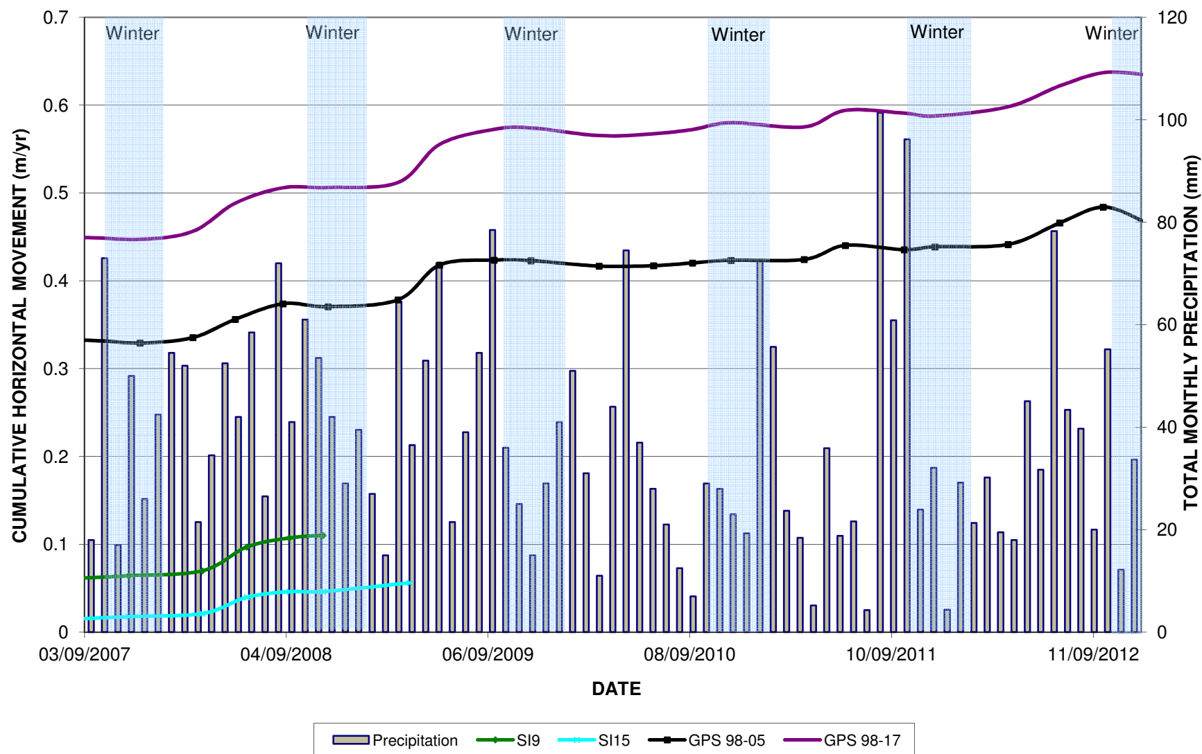
Figure G5 - Cumulative Ground Movement vs. Total Monthly Precipitation (Quesnel)
