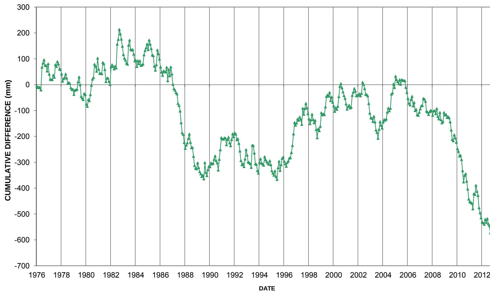
Figure F4 - Total Monthly Precipitation - Cumulative Difference - 1976 to 2012 (Environment Canada - Quesnel)
