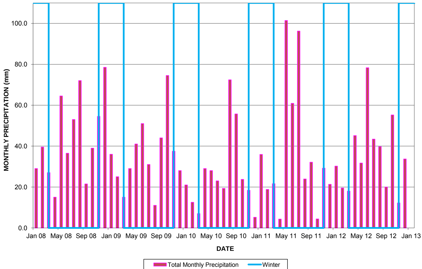
Figure F1 - Total Monthly Precipitation (Environment Canada-Quesnel Station)
