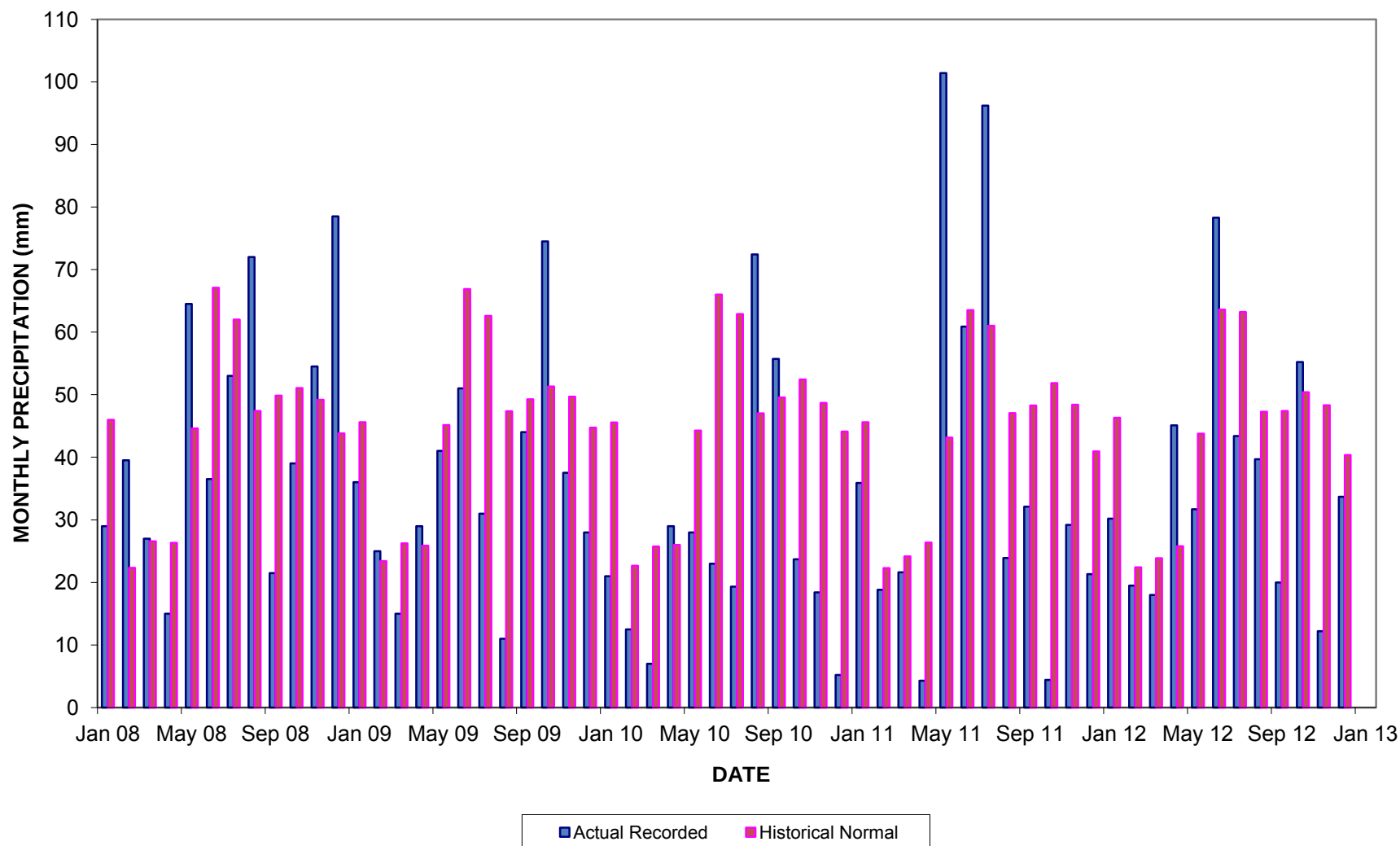
Figure F3 - Total Monthly Precipitation - 2008 to 2012 (Environment Canada - Quesnel)
