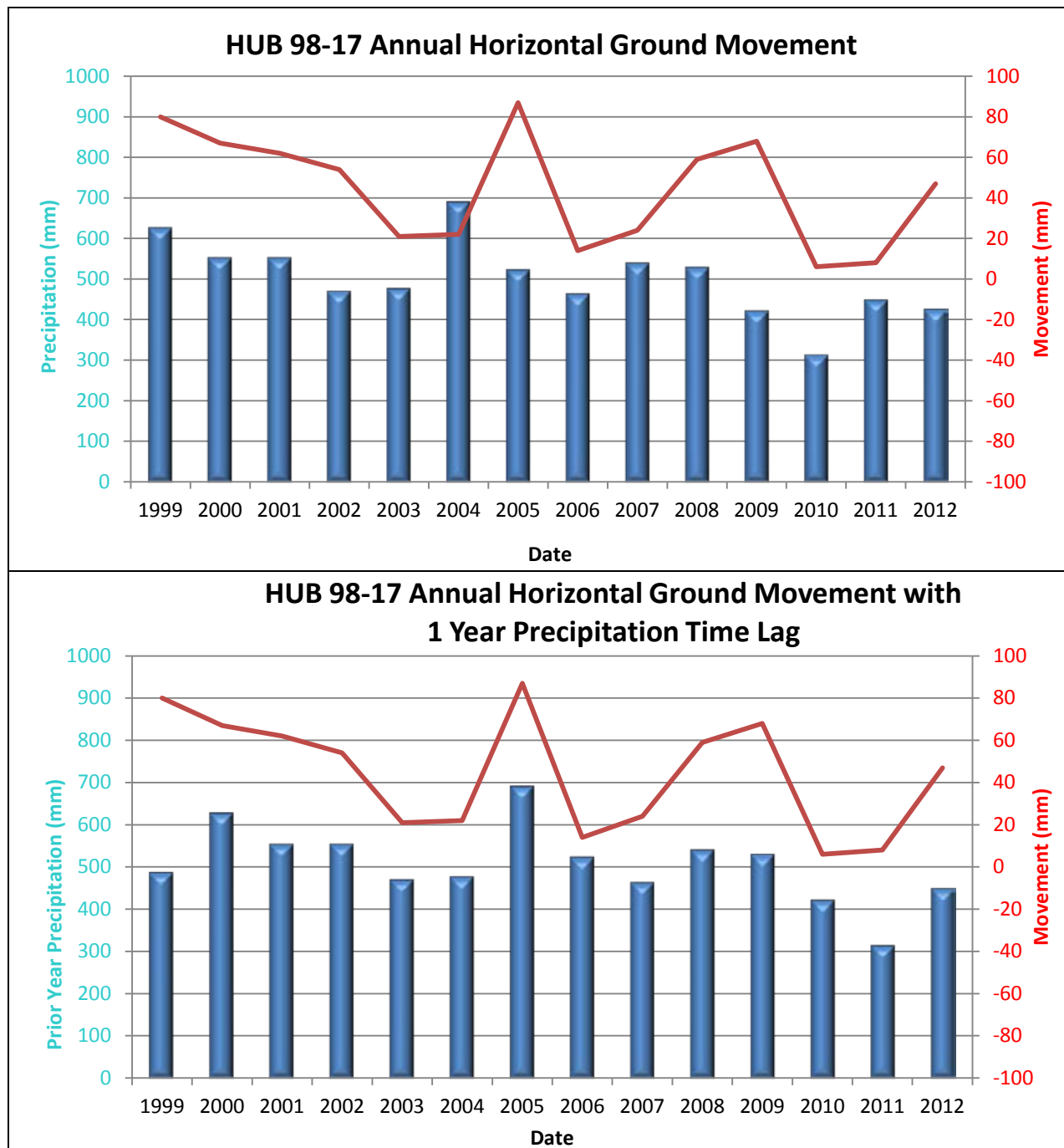
Figure G9 - Horizontal Movement Relative to Precipitation
