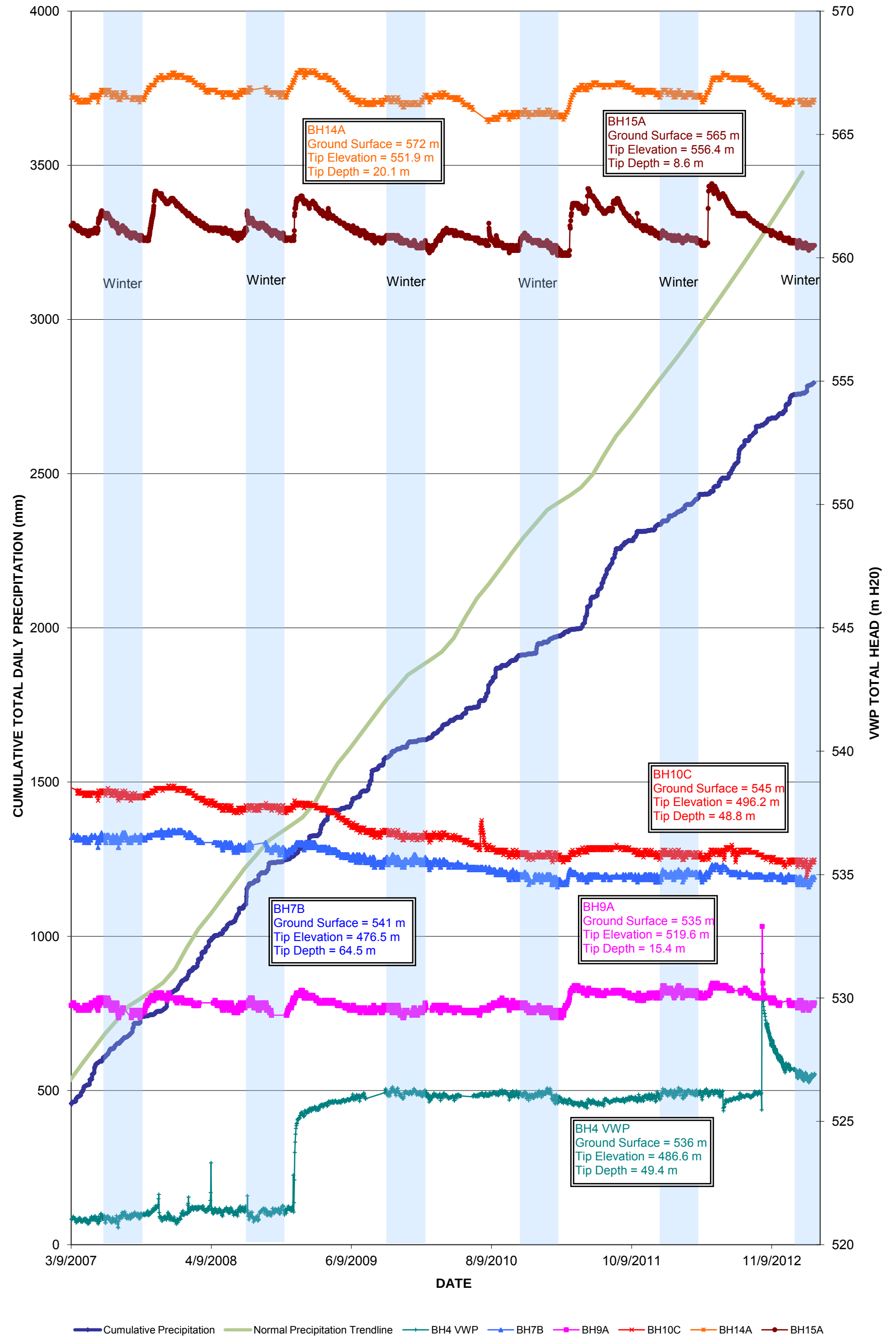
Figure G2 - Cumulative Total Daily Precipitation (Quesnel) vs. Groundwater Elevation
