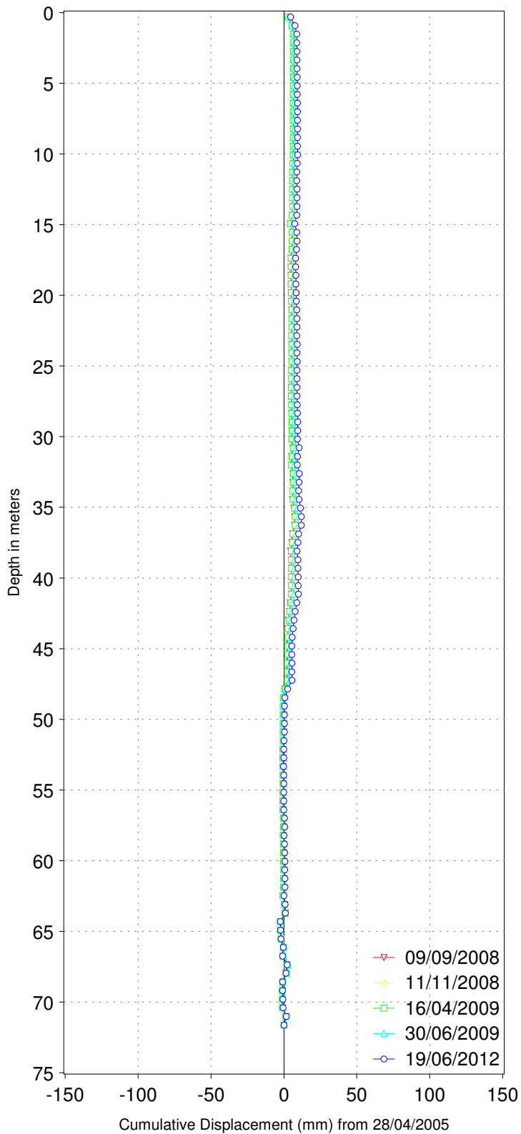
SI-8, A-Axis, Cumulative
