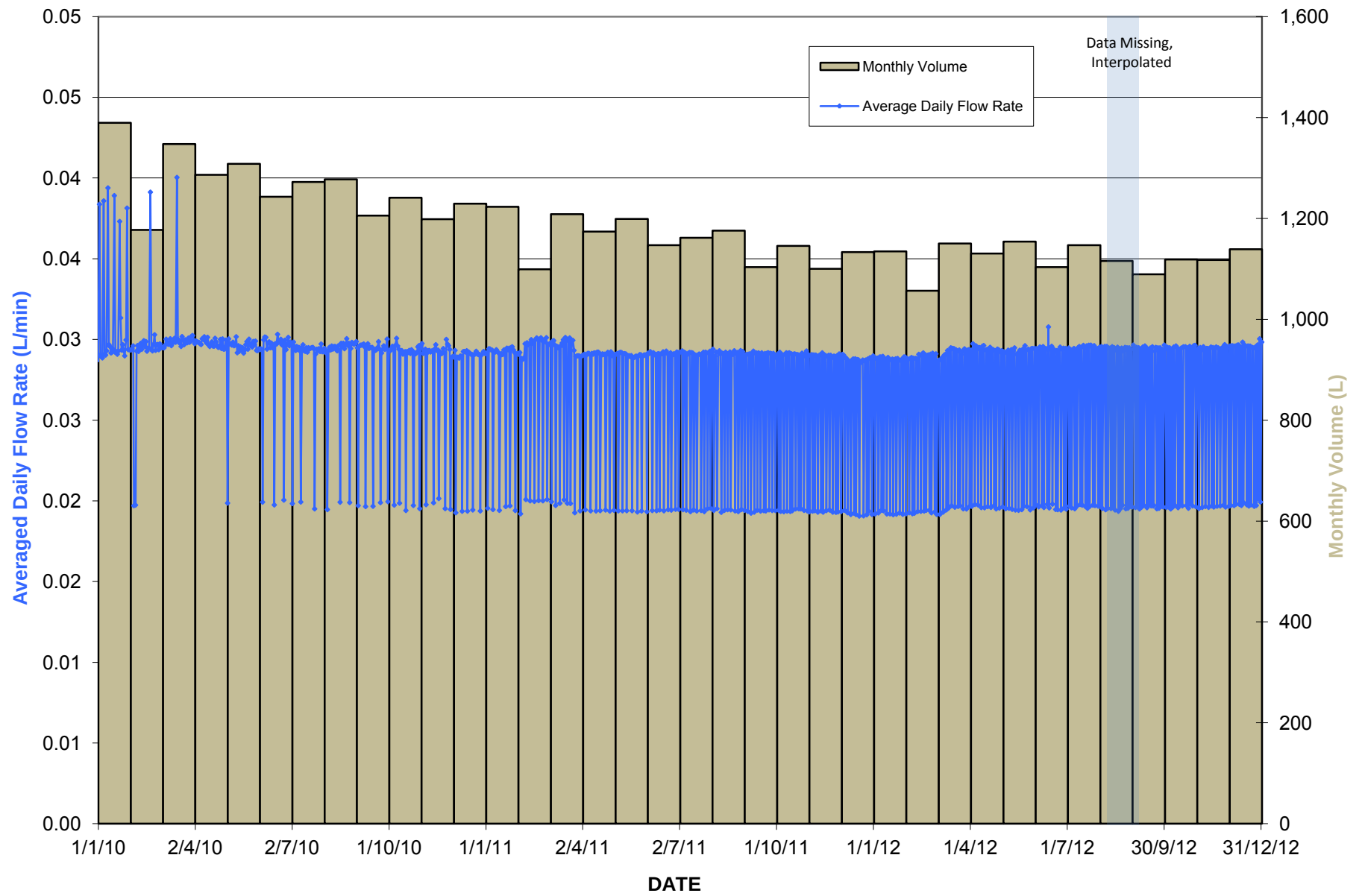
Averaged Daily Flow Rate and Monthly Discharged Volume for PW1
