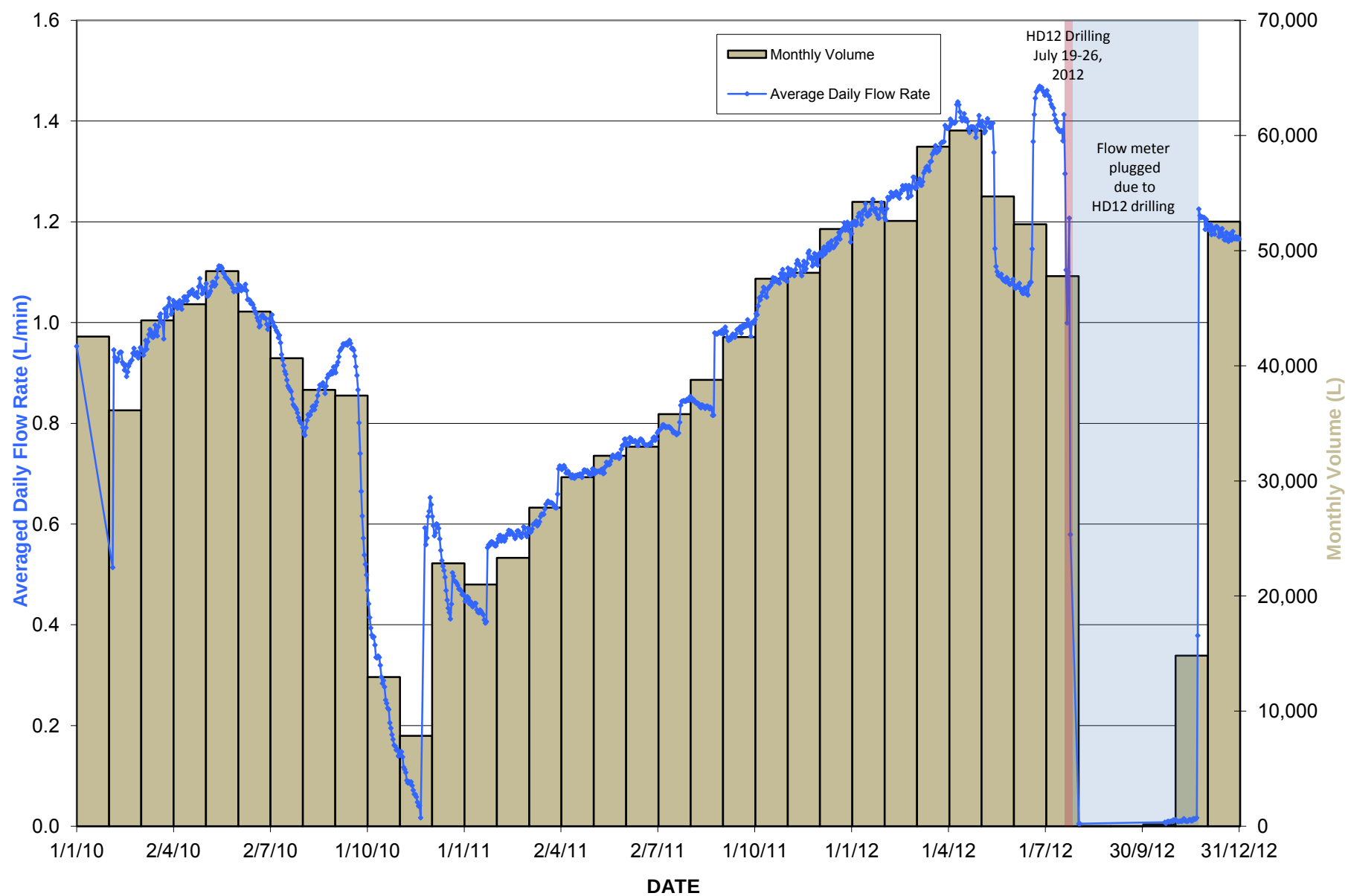
Averaged Daily Flow Rate and Monthly Discharged Volume for HD4
