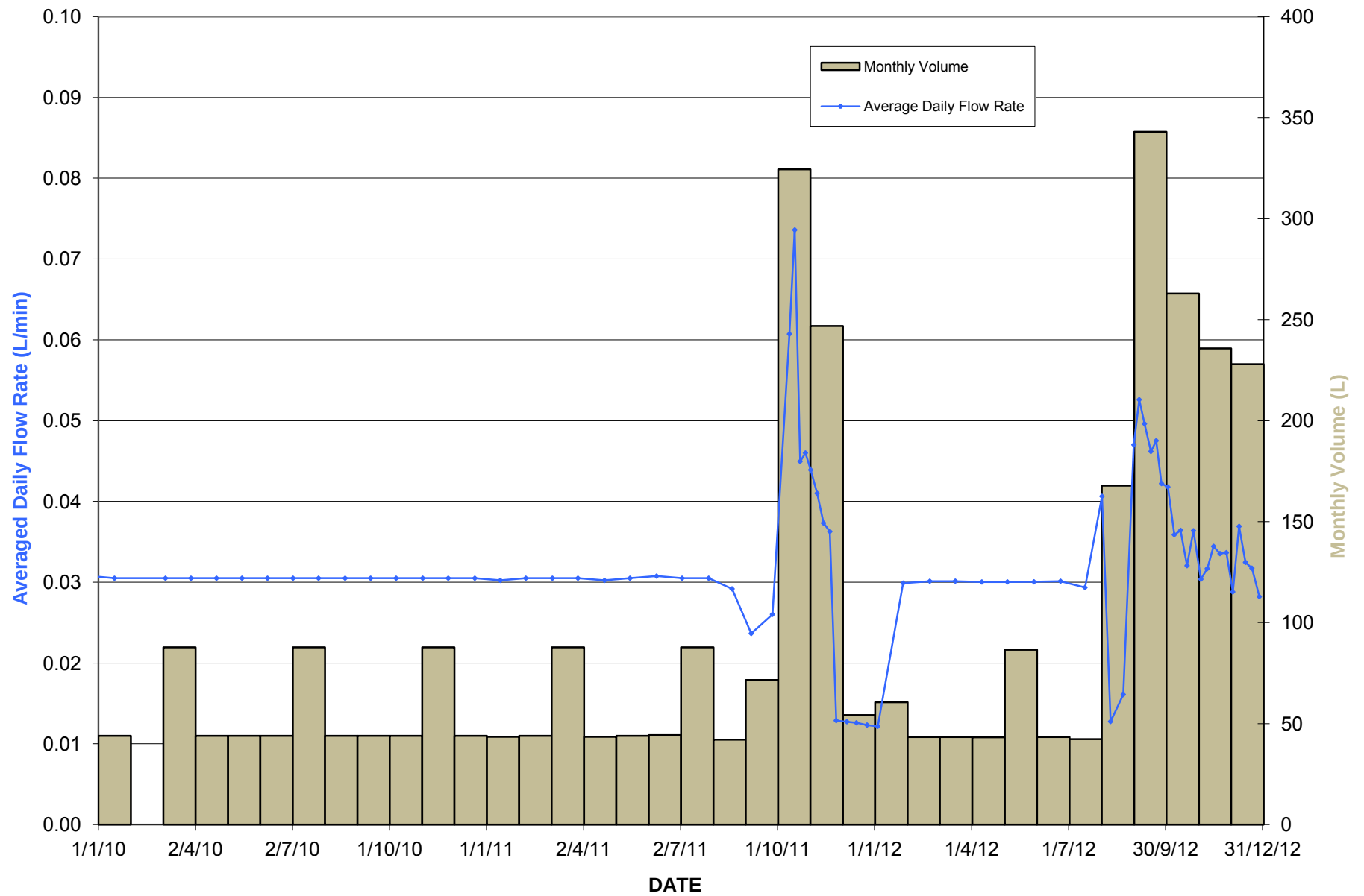
Averaged Daily Flow Rate and Monthly Discharged Volume for PW5
