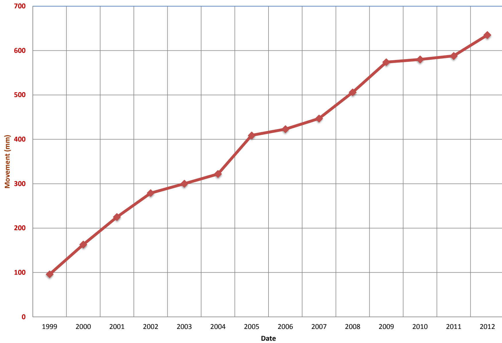
Figure A1: HUB 98-17 Total Horizontal Ground Movement
