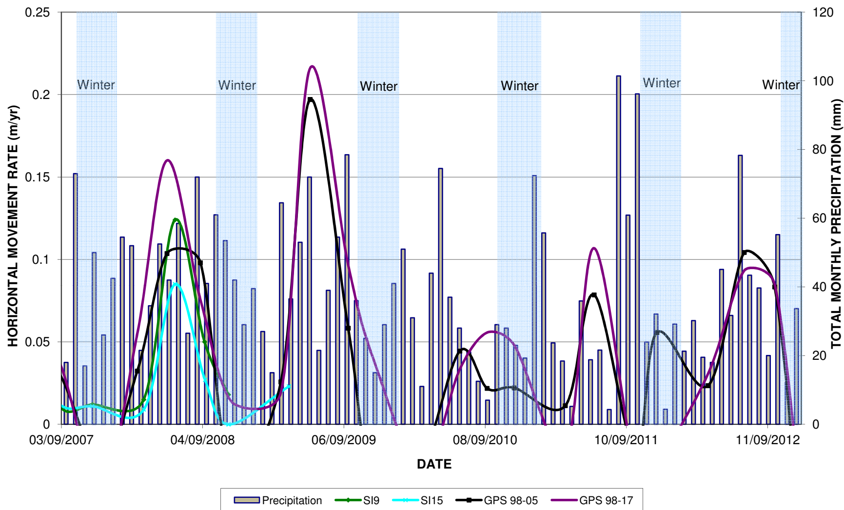
Figure G3 - Incremental Ground Movement Rate vs. Total Monthly Precipitation (Quesnel)
