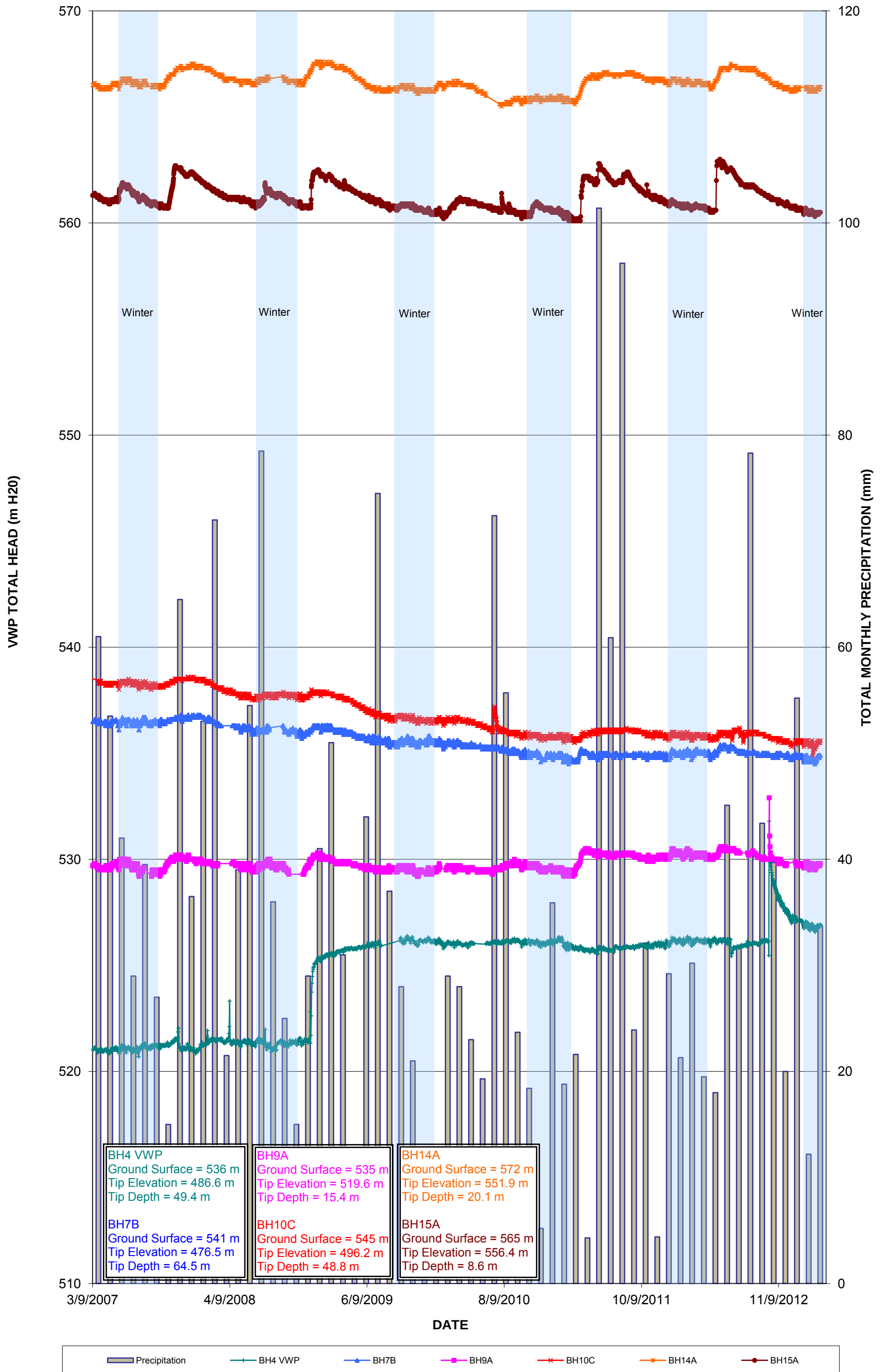
Figure G1 - Total Monthly Precipitation (Quesnel) vs. Groundwater Elevation
