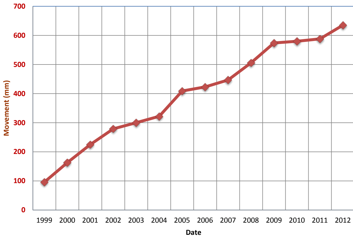
Figure A1: Hub 98-17 Total Horizontal Ground Movement
