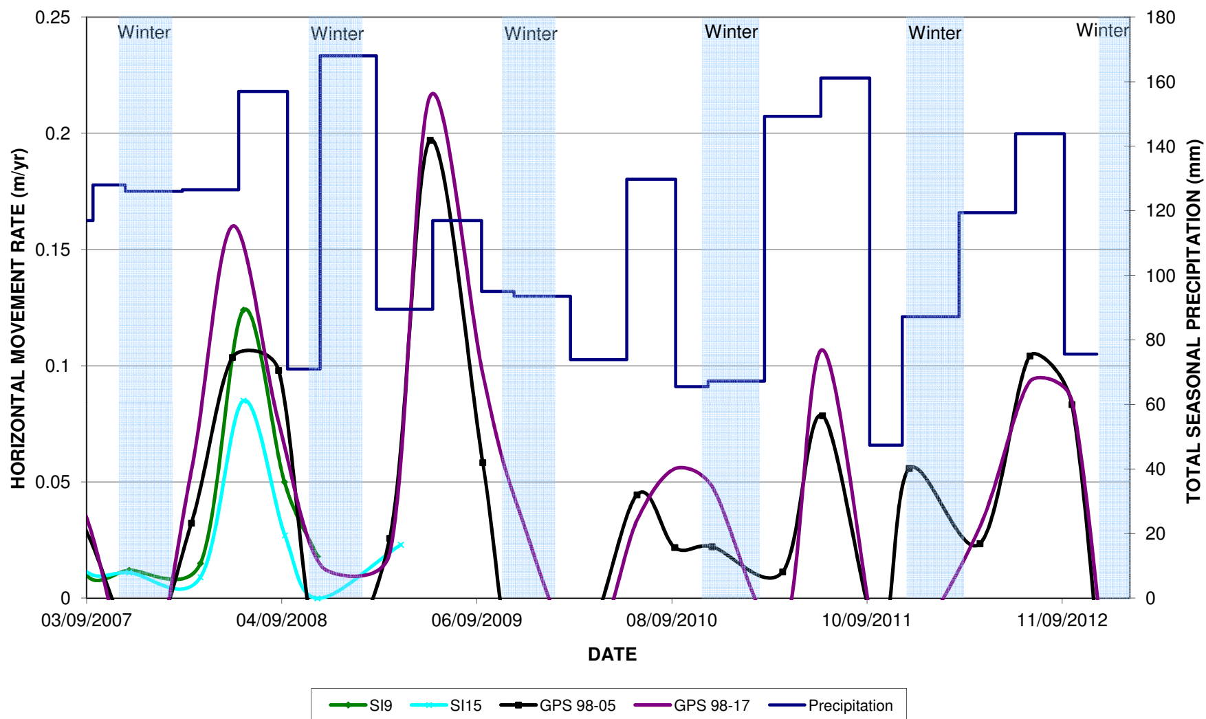
Figure G4 - Incremental Ground Movement Rate vs. Total Seasonal Precipitation (Quesnel)
