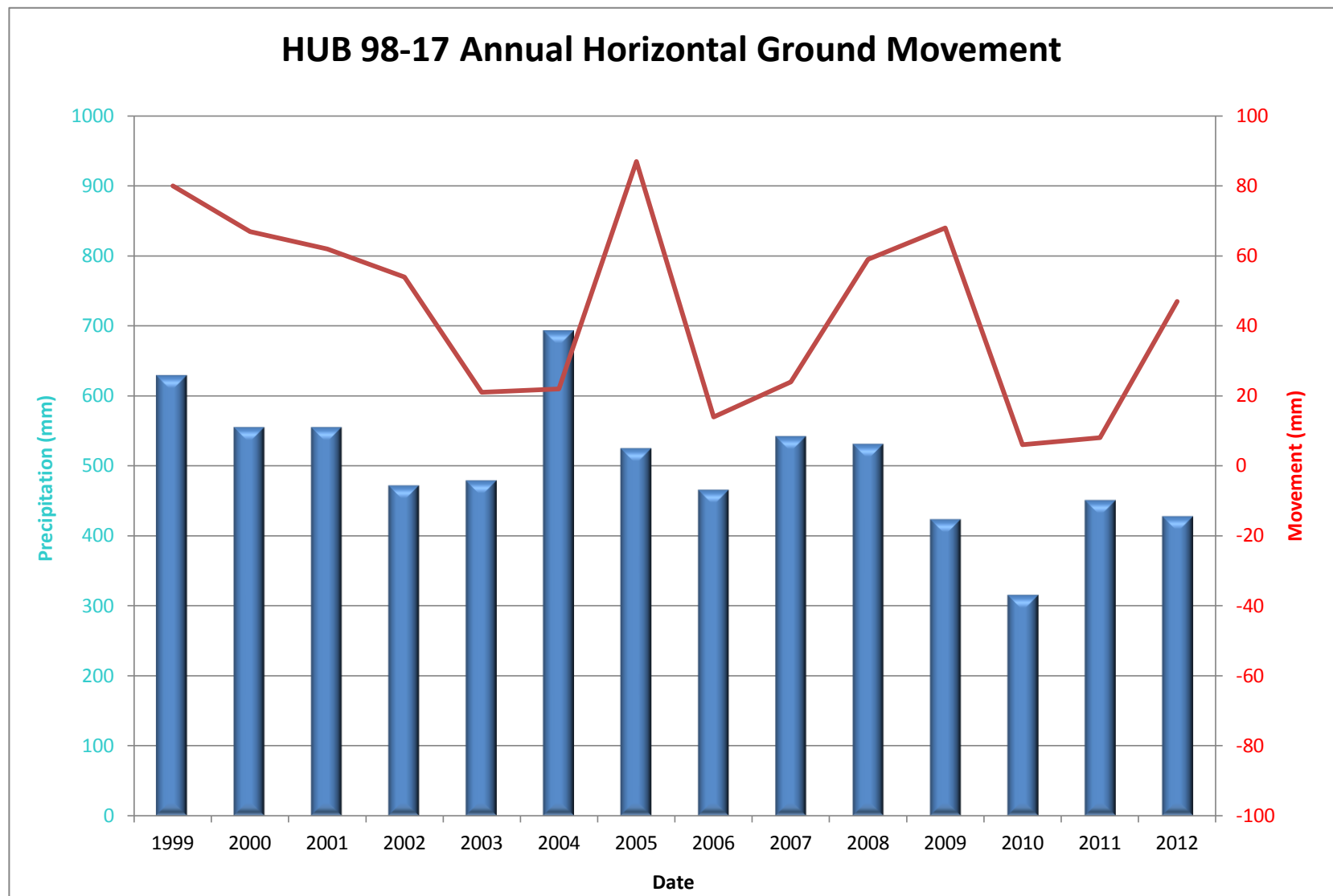
Figure G9 - Horizontal Movement Relative to Precipitation
