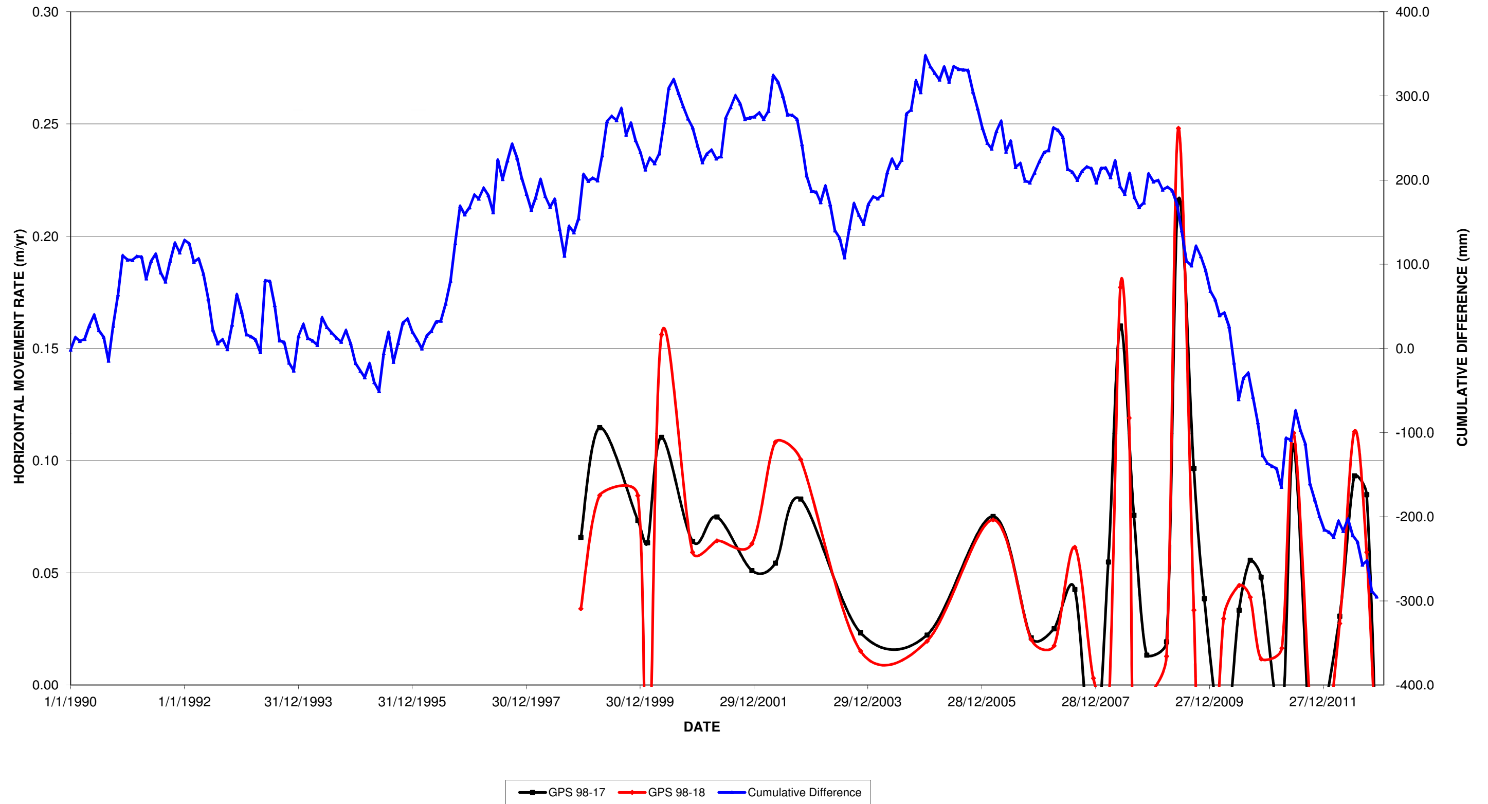
Figure G6 - Incremental Ground Movement Rate vs. Cumulative Difference - Total Monthly Precipitation (Quesnel)
