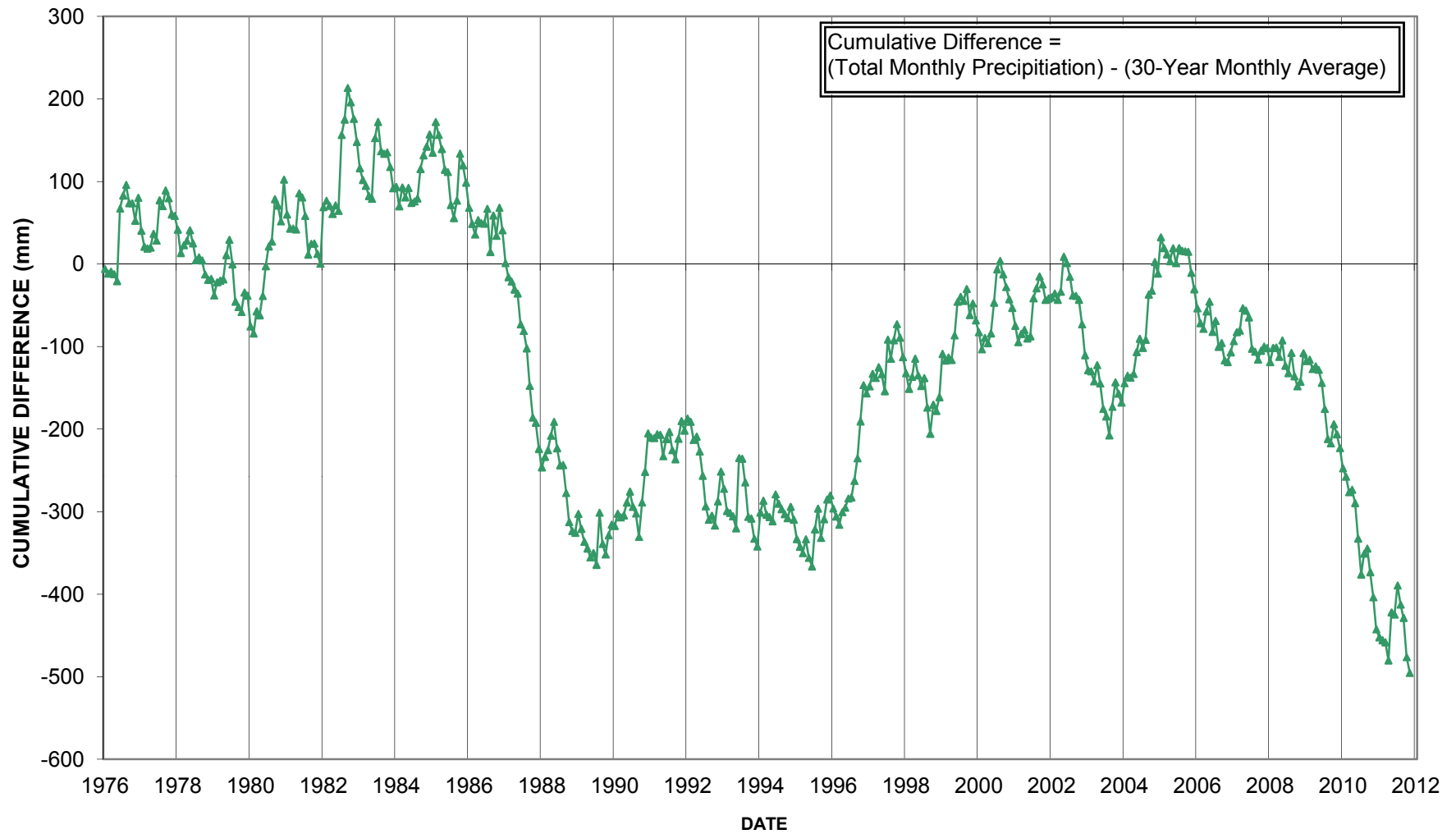
Figure F4 - Total Monthly Precipitation - Cumulative Difference - 1976 to 2011 (Environment Canada - Quesnel AWOS)
