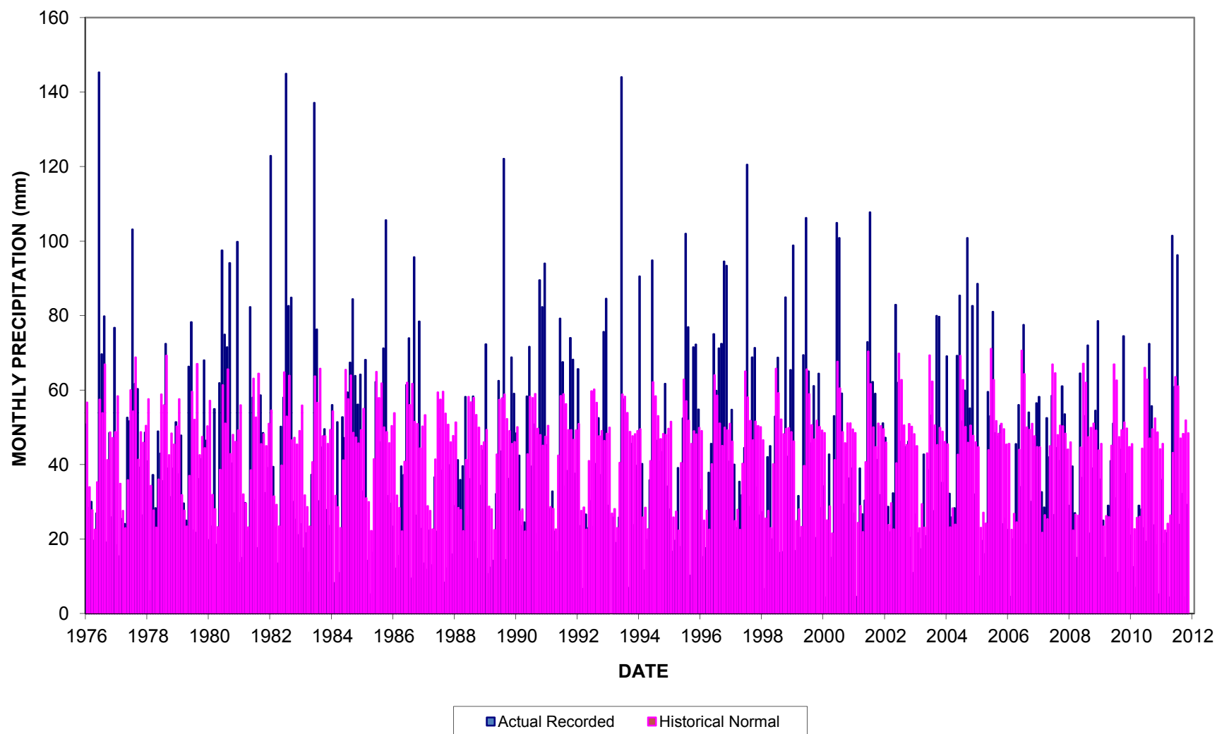
Figure F3 - Total Monthly Precipitation - 1976 to 2011 (Environment Canada - Quesnel AWOS)
